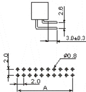
RECOMMENDED P.C BOARD HOLE LAYOUT
