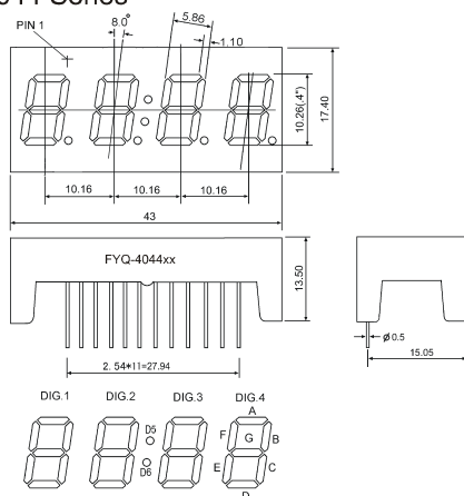
FYQ-4044 Series
